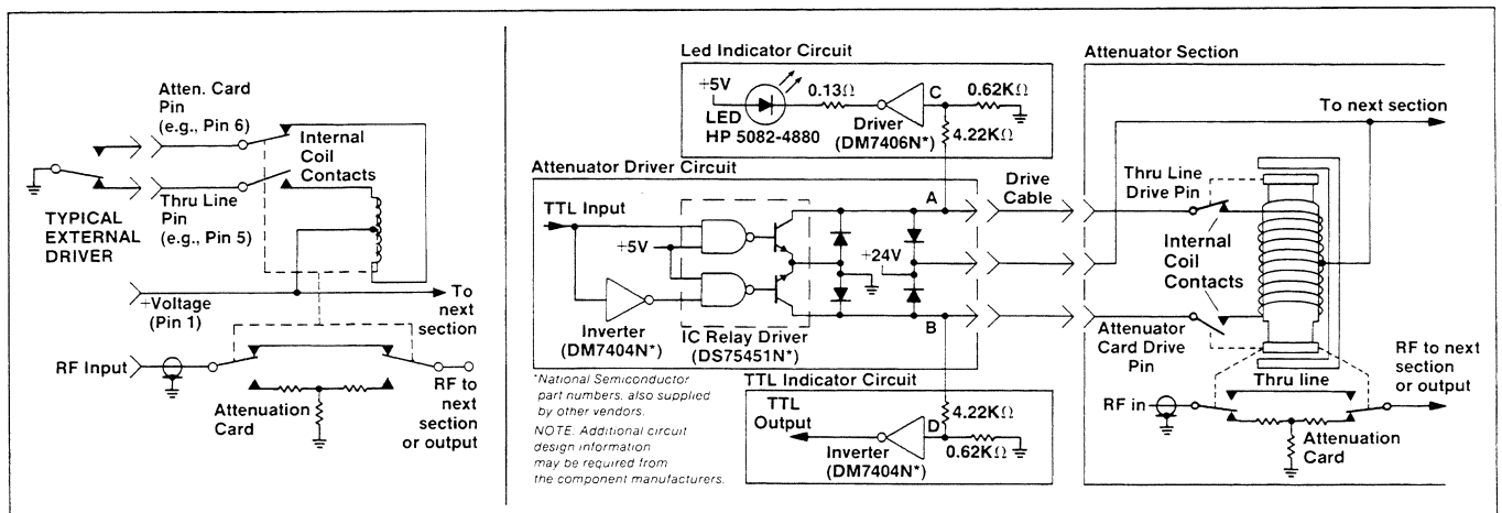
Figure 5. Driver and indicator circuits for one section of an HP 33320, 1, 2, 3, G/H/K
